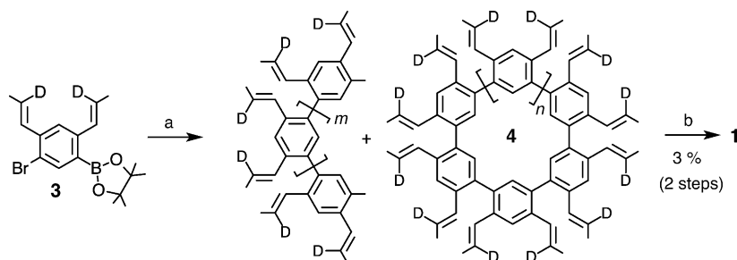
Scheme 2. a) [\text{Pd}\{\text{P}(\text{p-tol})_3\}_3] , \text{K}_2\text{CO}_3 , THF/ \text{H}_2\text{O} , b) Grubbs 2nd generation catalyst, 1,2,4-trichlorobenzene, toluene, 70 °C ( 4 , n=2 ).
